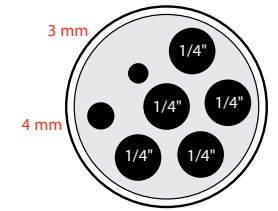
Multi-hole M05
